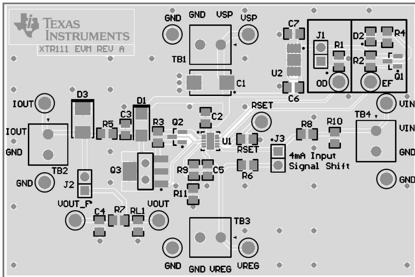
Figure 5. PCB Layout
