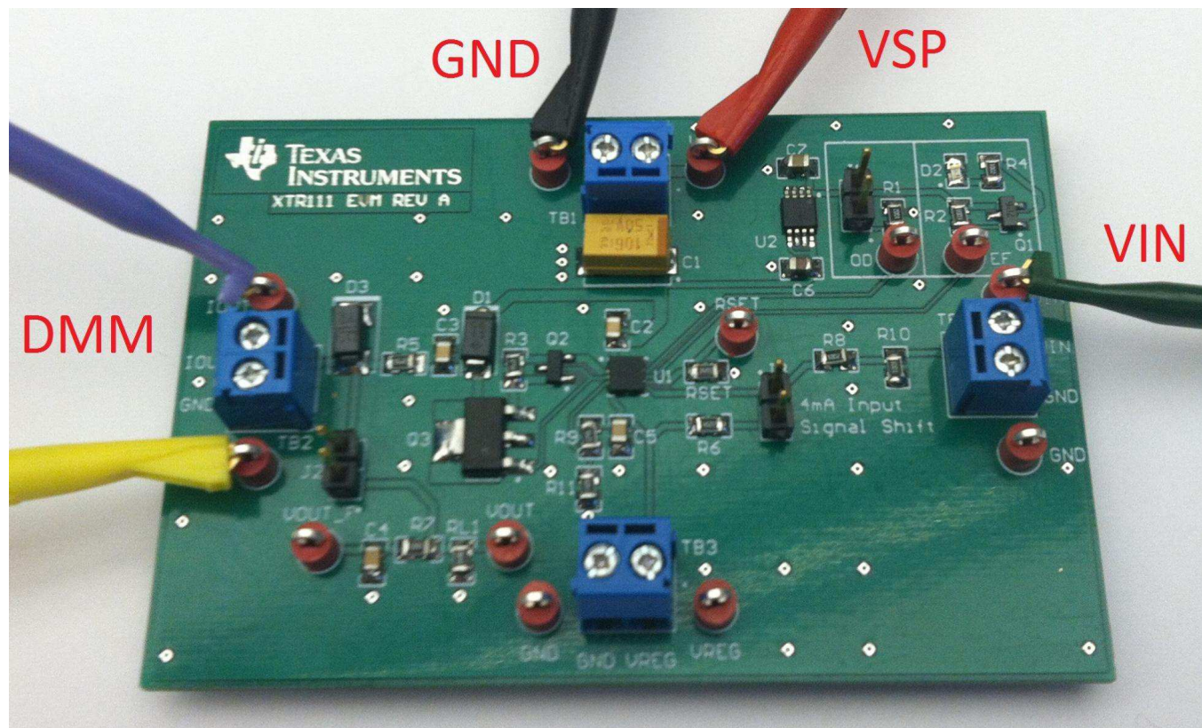
Figure 2. Current Output Setup
